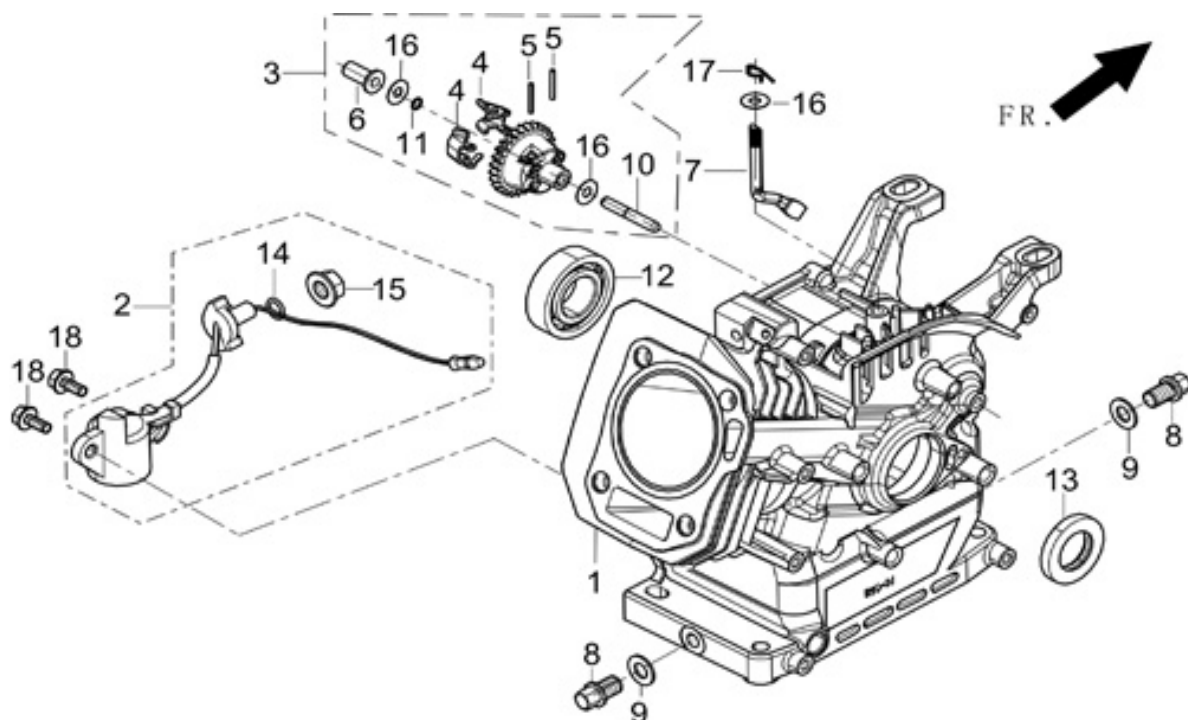
FIG.2 CRANKCASE. / GEAR ASSY, GOVERNOR. (E02)
