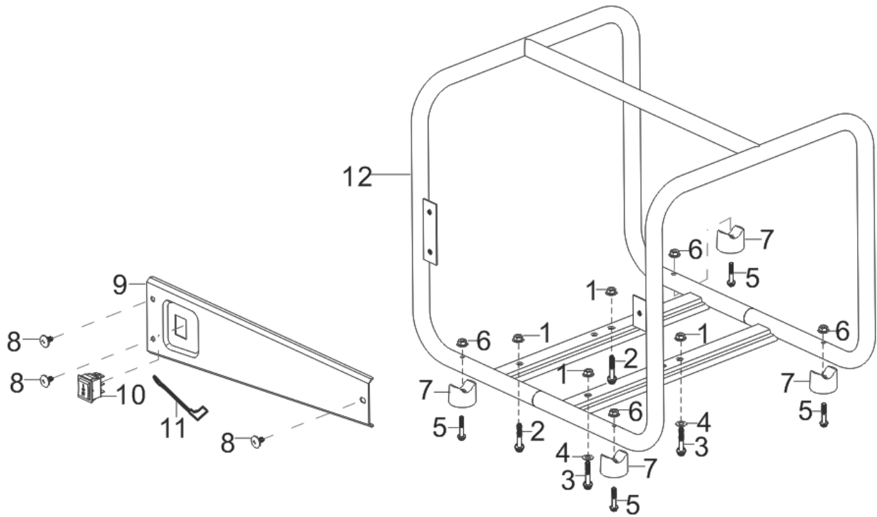
FIG.16 FRAME ASSY, ENGINE (E16)
