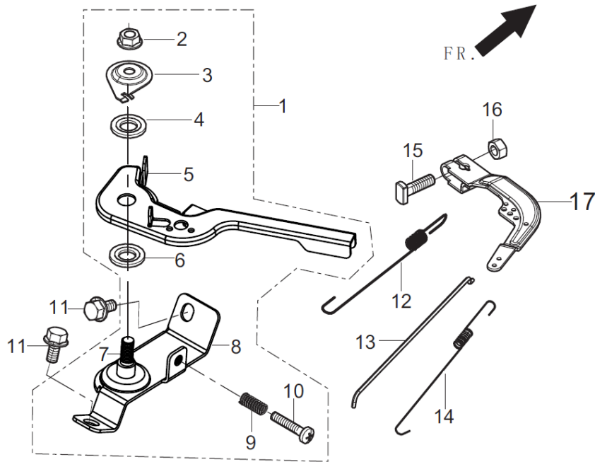
FIG.14 CONTROL ASSY, THROTTLE (E14 )
