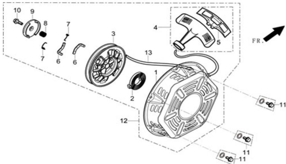
FIG.7 STARTER,RECOIL ( E07 )
