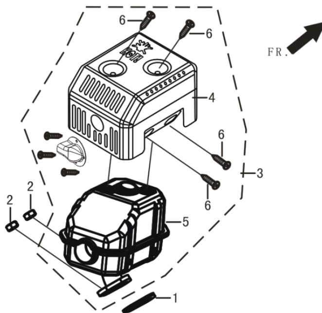
FIG.11 MUFFLER ASSY. ( E11 )
