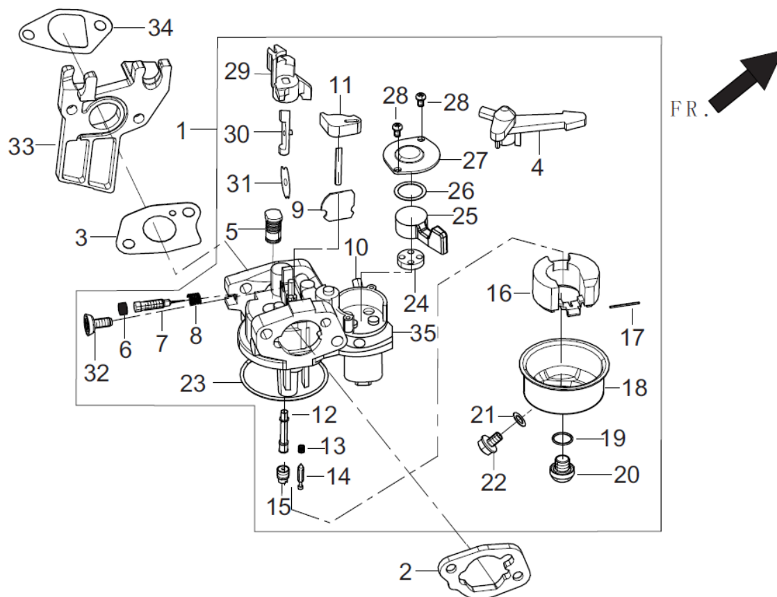
FIG.9 CARBURETOR ASSY. ( E09 )
