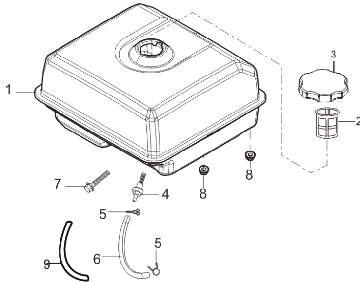
FIG.12 TANK ASSY, FUEL ( E12 )
