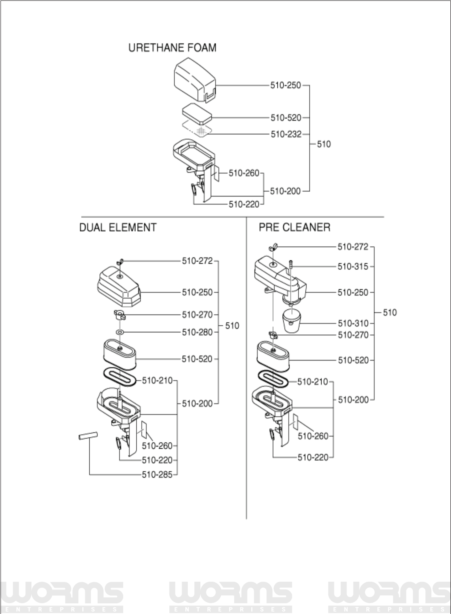
FIG. 315 INTAKE and EXHAUST GROUP
