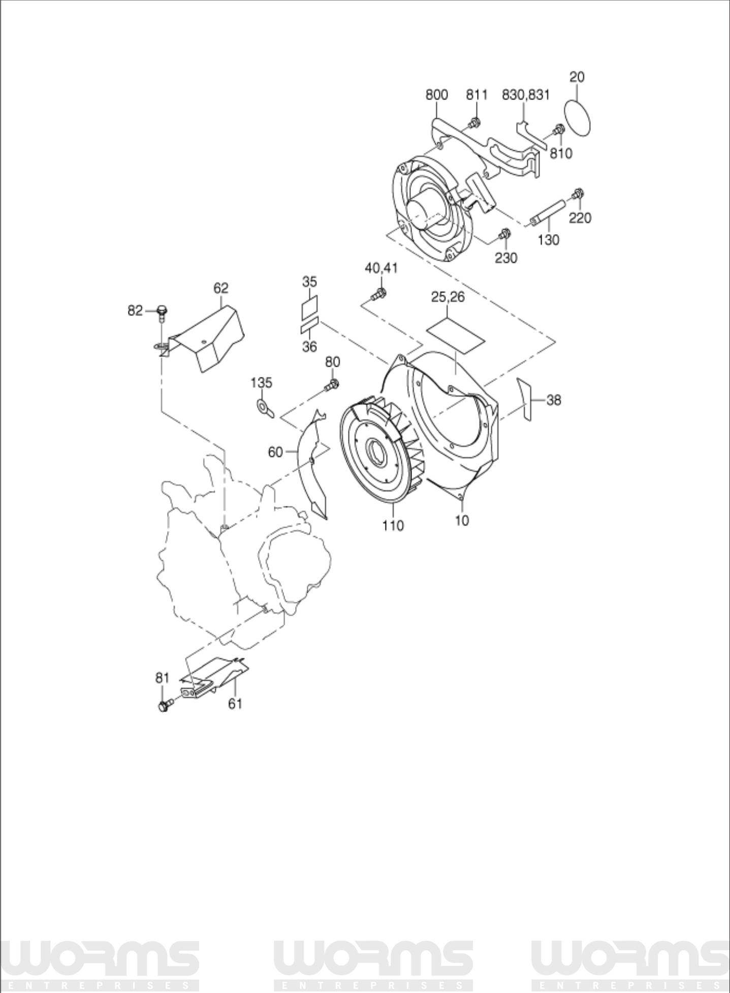
FIG. 500 COOLING and STARTING GROUP
