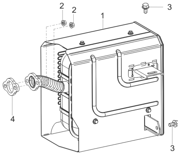
FIG.11 MUFFLER ASSY.(F04)
