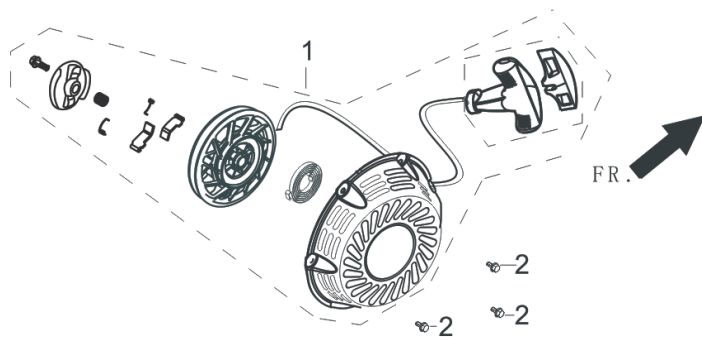
FIG.7 STARTER (E08)
