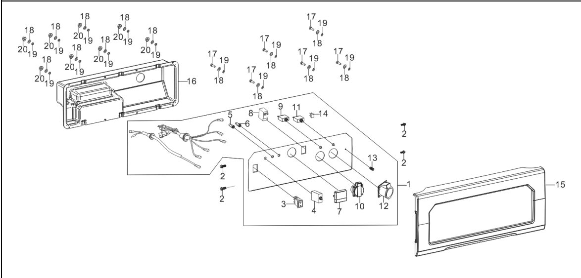
FIG.16 PANEL SUBASSEMBLY, CONTROL (F62)
