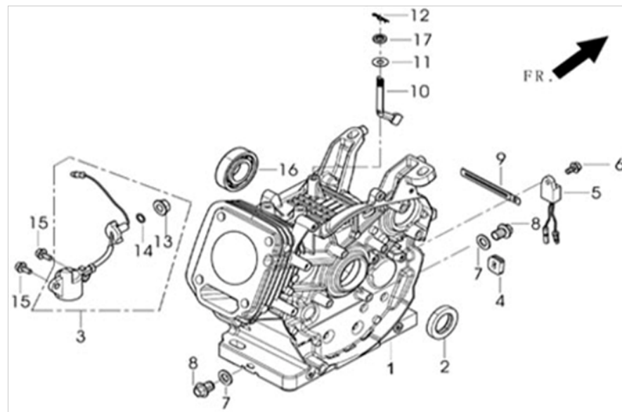
FIG.2 CRANKCASE (E17)
