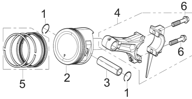
FIG.5 PISTON/CONNECTING ROD (E03)
