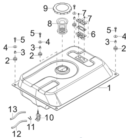
FIG.12 TANK, FUEL (F01)
