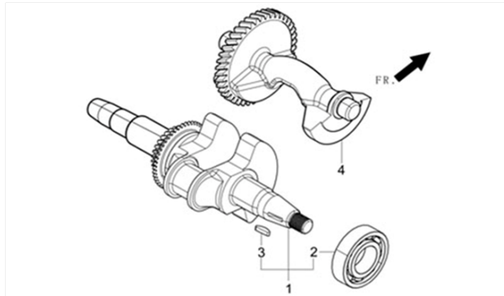
FIG.4 CRANKSHAFT ASSY.(E03)
