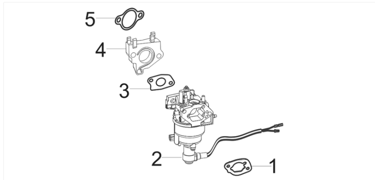
FIG.9 CARBURETOR ASSY.(E11)
