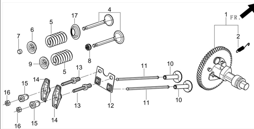
FIG.6 CAMSHAFT ASSY. (E05)
