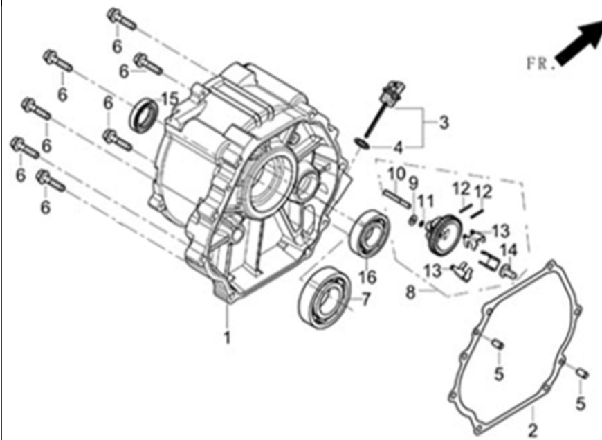
FIG.3 COVER, CRANKCASE (E01)
