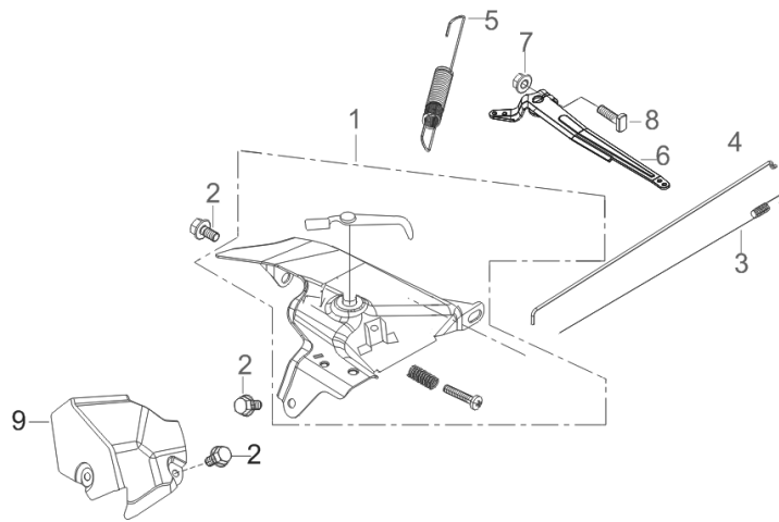
FIG.14 CONTORL ASSY.(E13)
