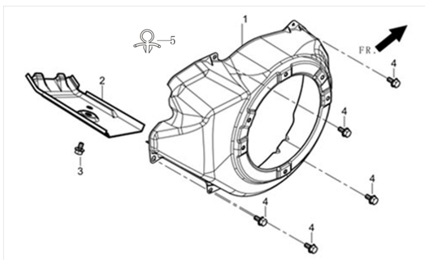
FIG.8 SHROUD (E14)
