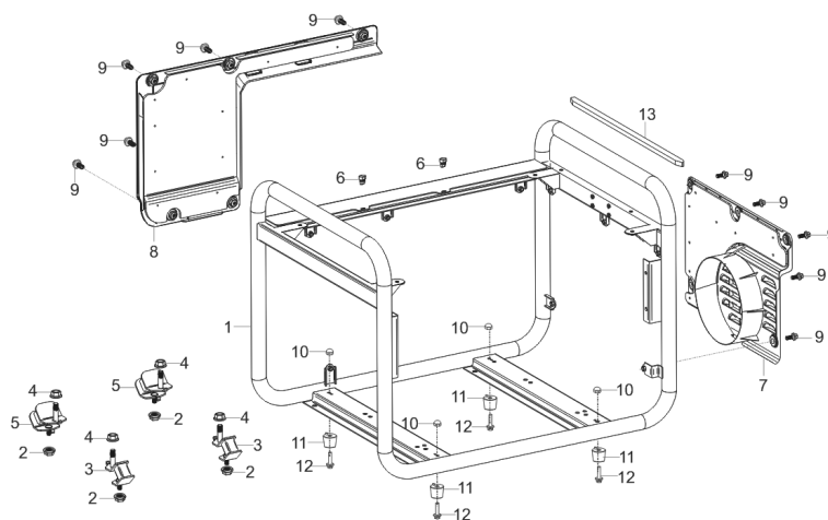
FIG.15 FRAME, ENGINE (F61)
