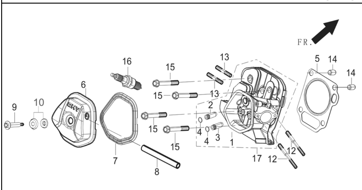
FIG.1 CYLINDER HEAD , CYLINDER COVER ASSY (E04)
