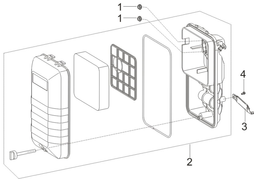
FIG.10 AIR CLEANER (F02)
