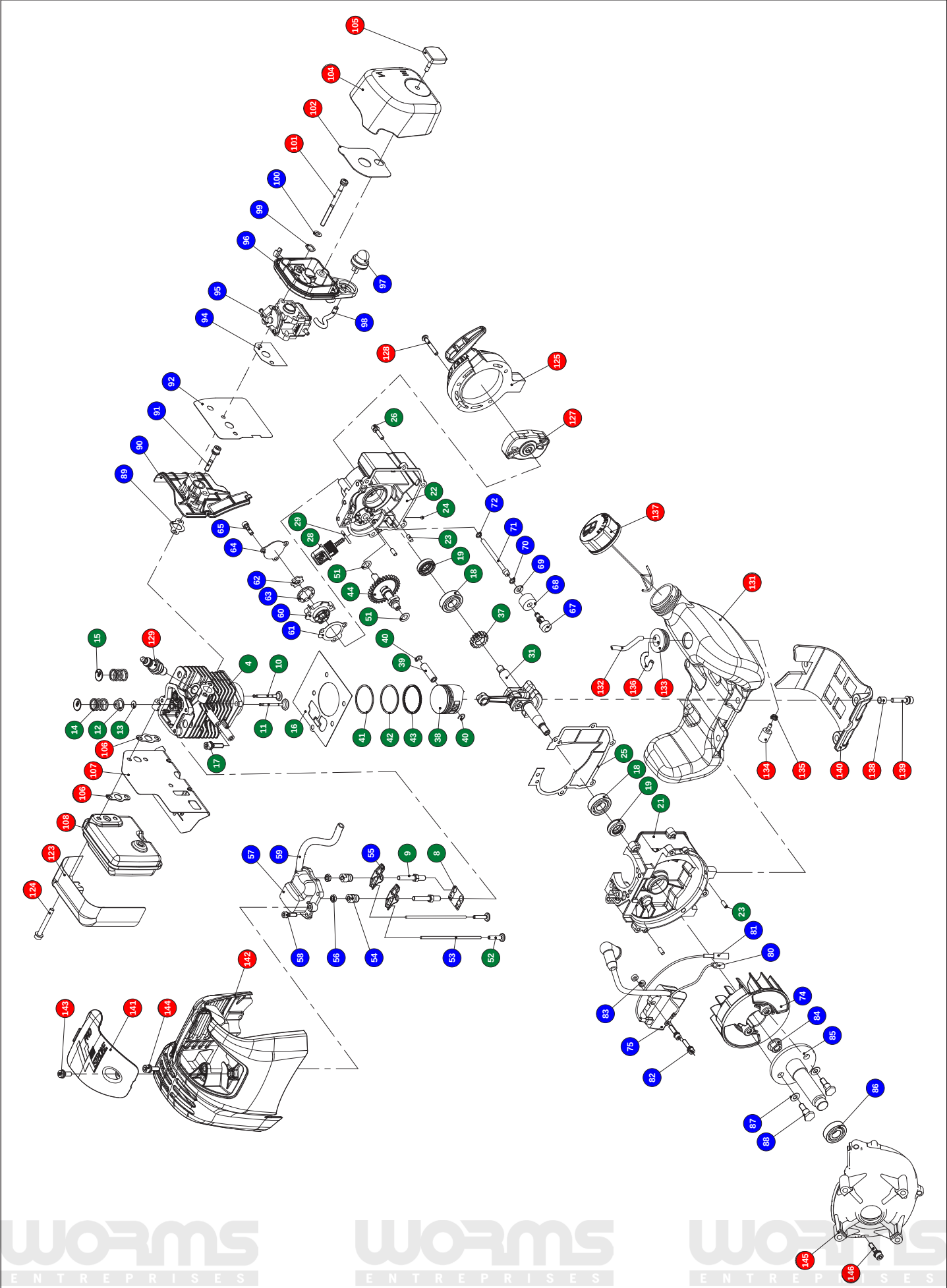
FIG. 2 ENGINE
